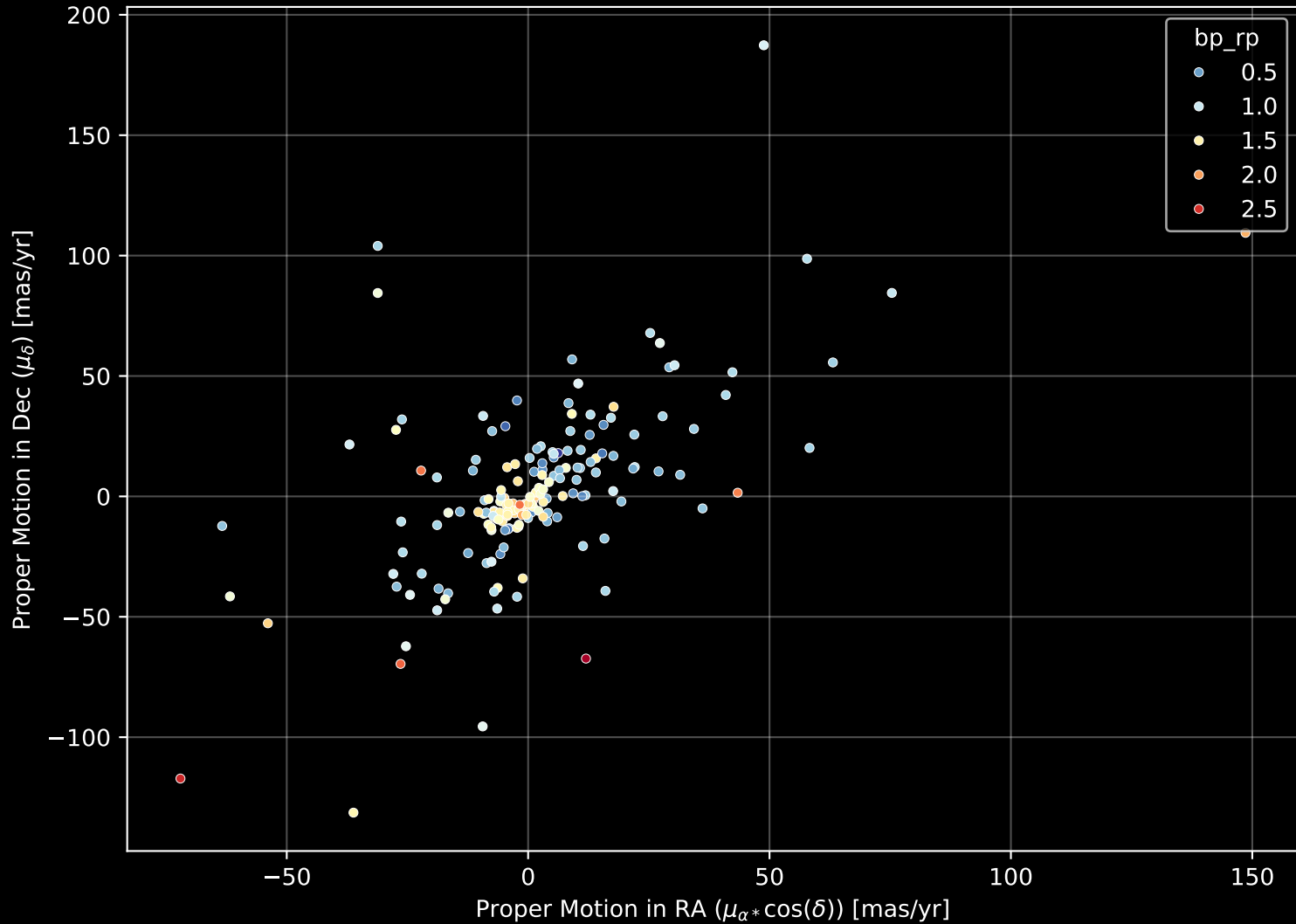
APOGEE DR17 Field: [CVZTILE_101+20_btx] Proper Motion Diagram (n= 181)
