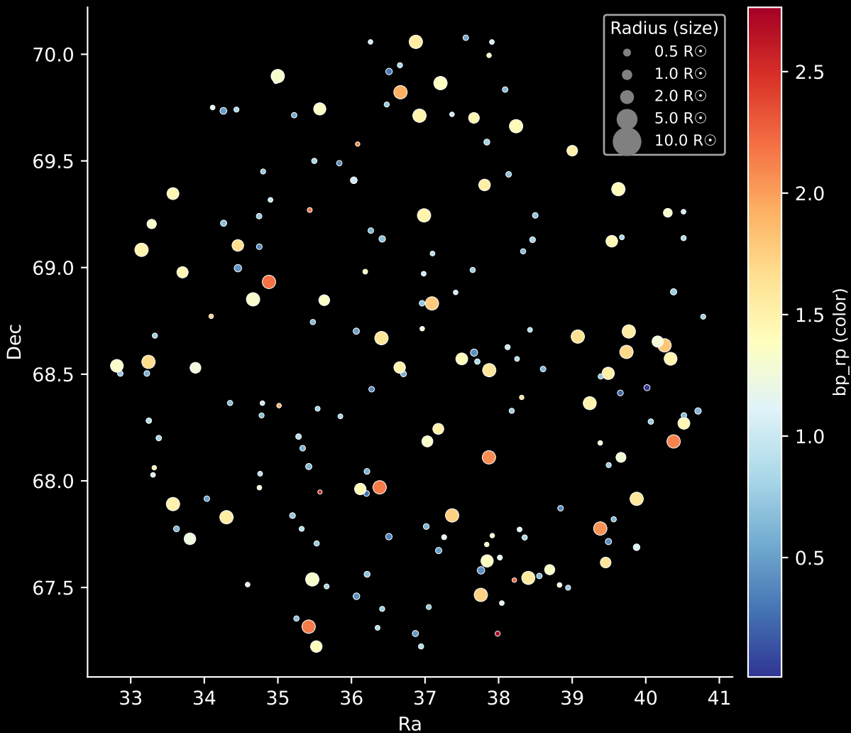
APOGEE DR17 Field: [CVZTILE_101+20_btx] Stars: 181
