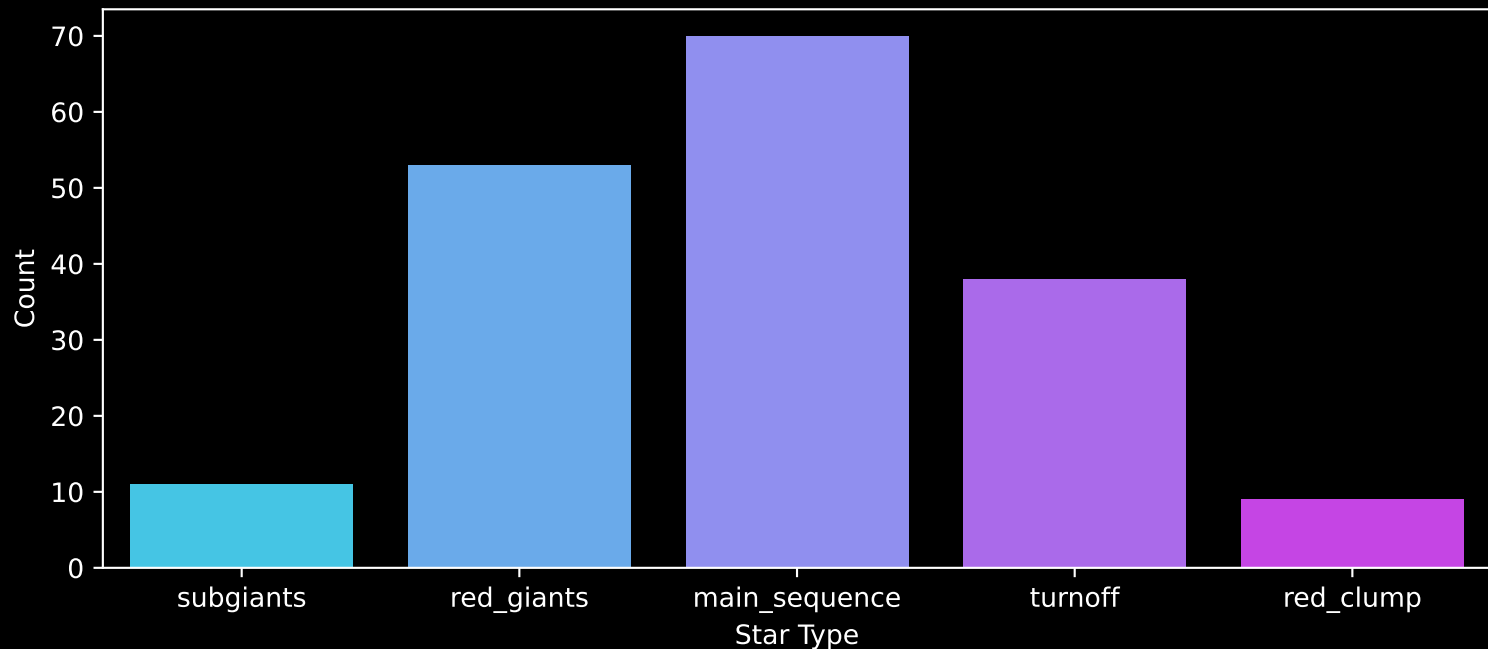
APOGEE DR17 Field: [CVZTILE_101+20_btx] Count plot of Star Type
