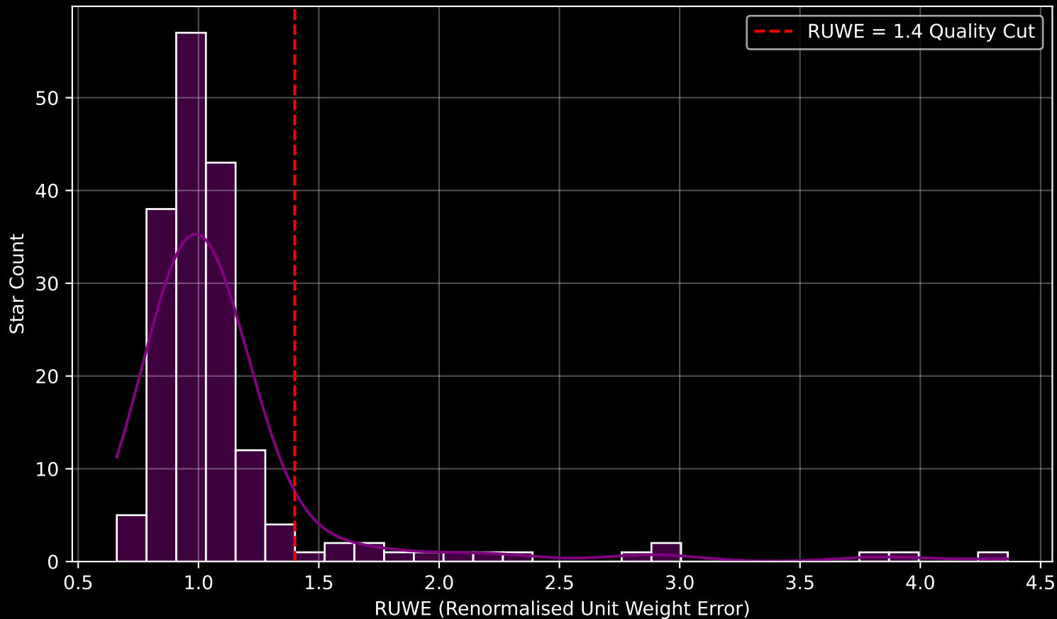
GAPOGEE DR17 Field [CVZTILE_101+20_btx] RUWE Distribution (n= 175)
