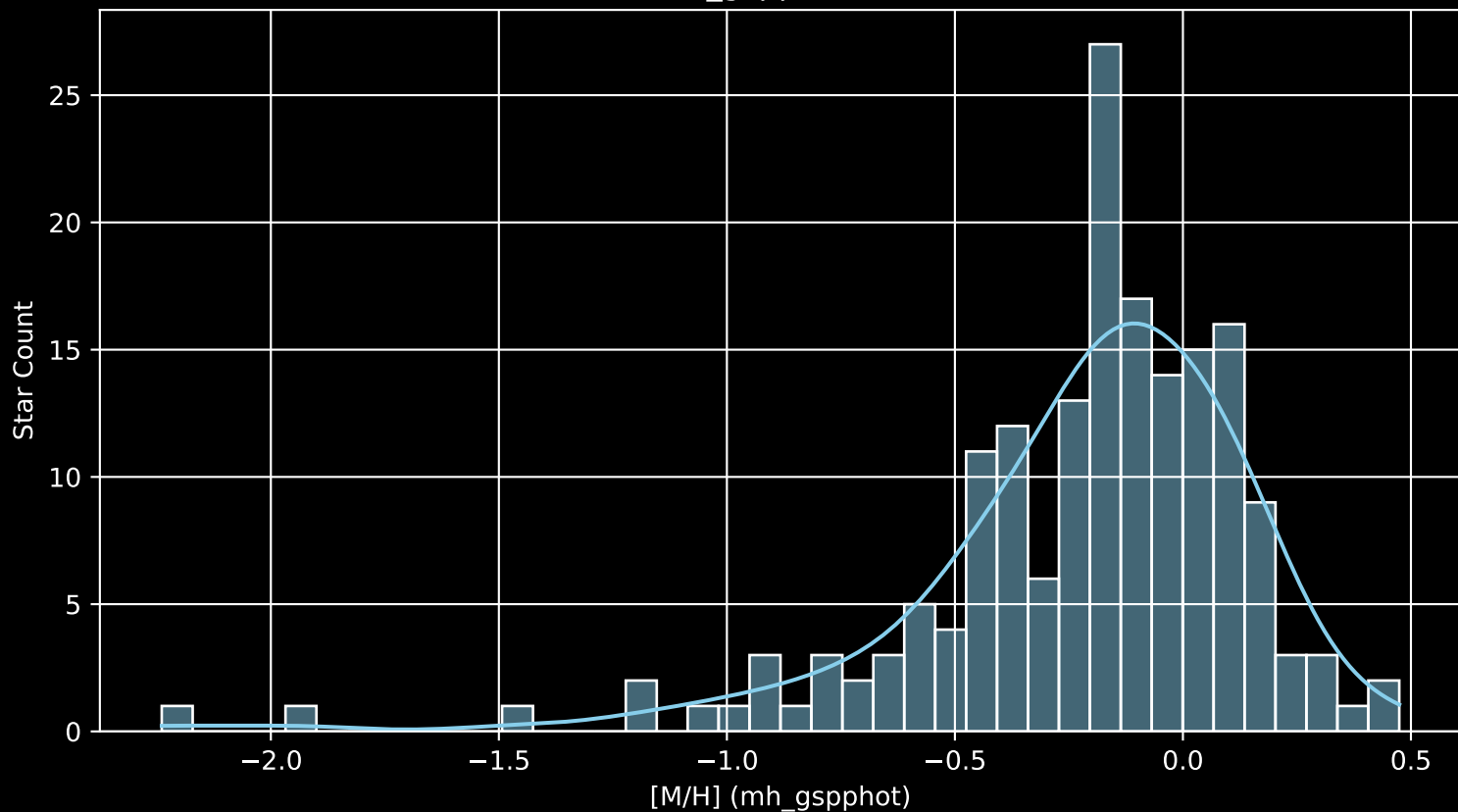
APOGEE DR17 Field: [CVZTILE_101+20_btx [M/H] (mh_gspphot) (n= 177)
