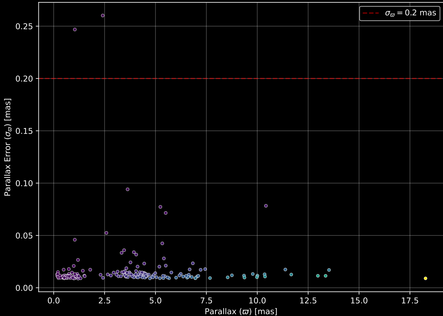
APOGEE DR17 Field: [CVZTILE_101+20_btx] Parallax Quality (n= 181)
