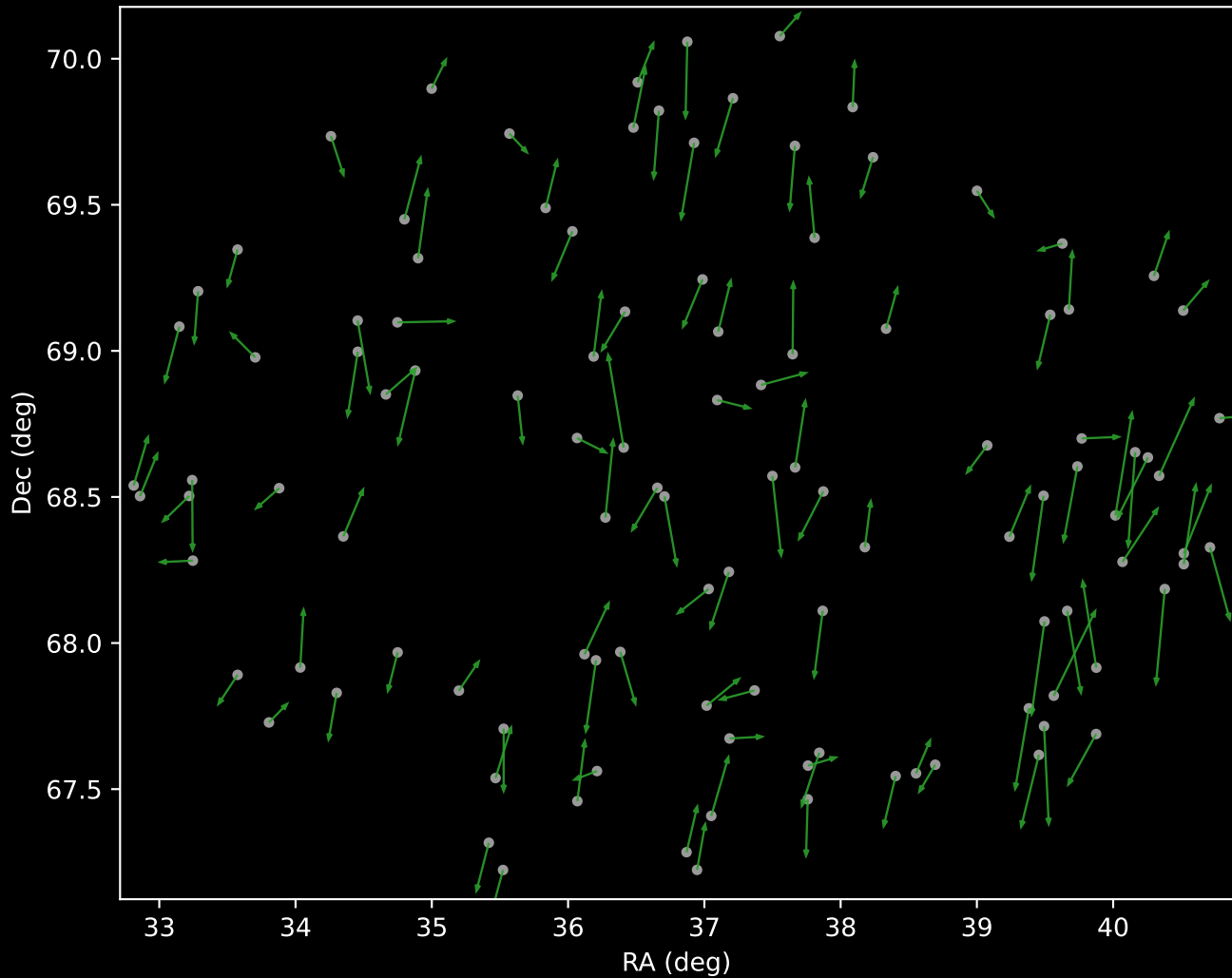
APOGEE DR17 Cluster 4 Proper Motion Vectors (n=111)
